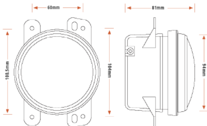
3.4" SIZING
