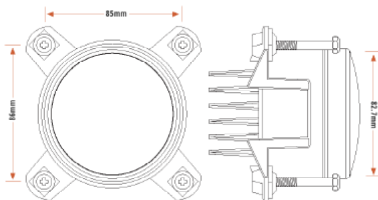
3.3" SIZING
