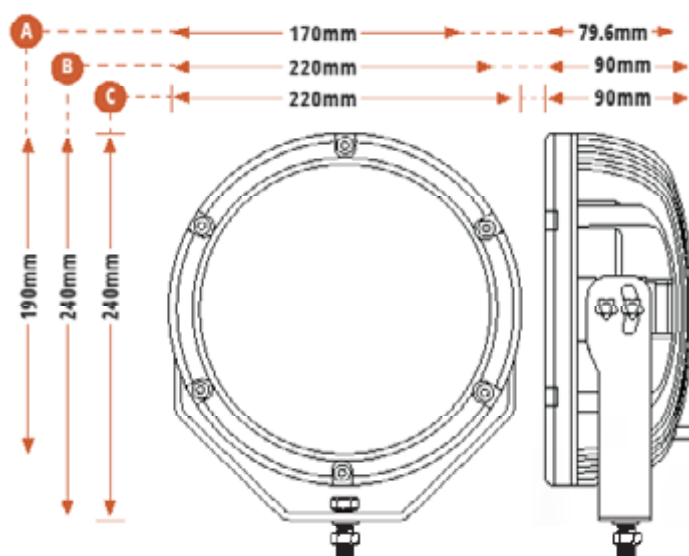
B EVFB180LED | 9"
