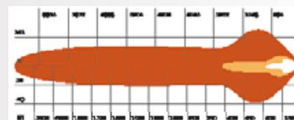
LASER + FLOOD EVSLD200LED
